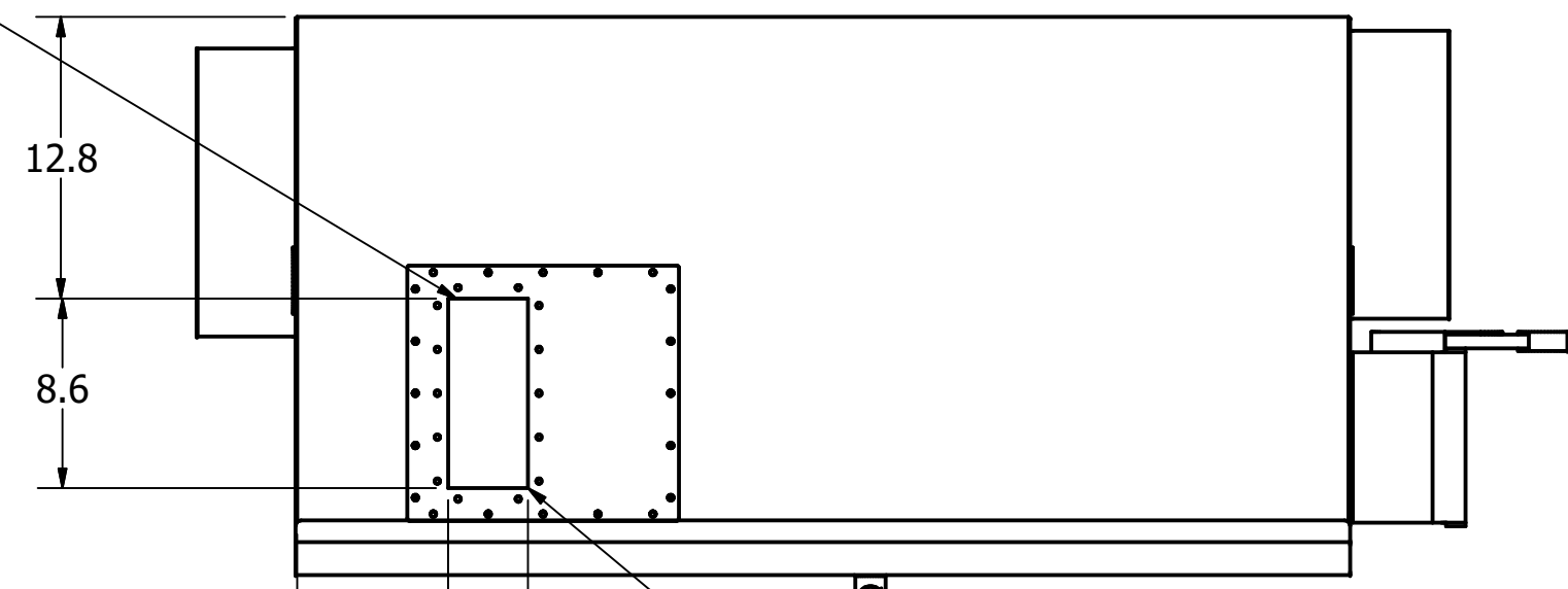
Front View Without Doors
