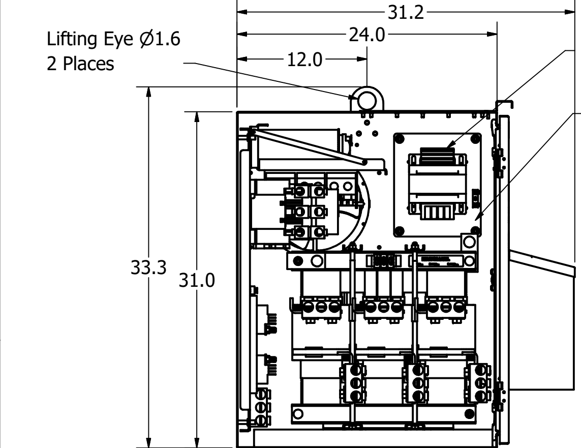
Side View Without Wall
